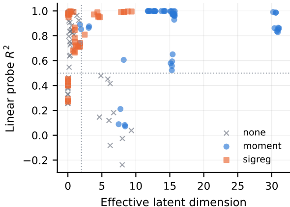
Two collapse axes: rank vs. decodability
